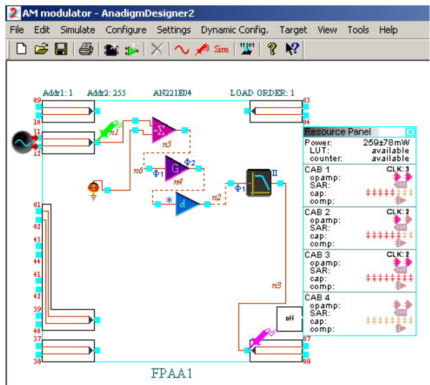
Design of Amplitude Modulator using FPAA
